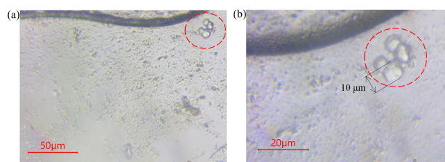
Fig. 8. Microphotographs depicting particles in the killing fluid: (a) 400x magnification; (b) 1000x magnification
