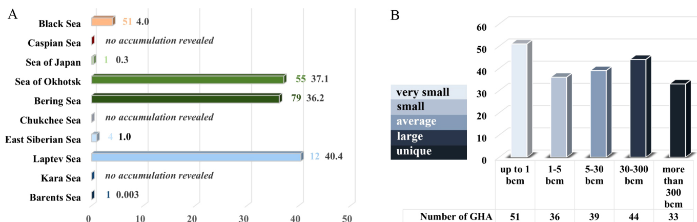
Figure 6. Histograms of the distribution of (A) the total local estimates of Q_1 (analogous to the Russian D1 category) for the predicted amount of methane in gas hydrate accumulations of filtration origin in Russian waters (black numbers, trillion \text{m}^3 ); colored numbers opposite the bars indicate the number of identified accumulations; and (B) a ranking of gas hydrate accumulations based on their resource, analogous to the ranking of conventional gas deposits by reserves.
