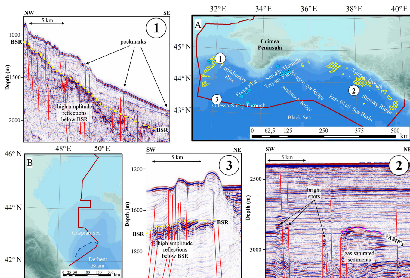
Figure 5. Gas hydrate accumulation of filtration origin in the Russian sector of the Black Sea (A), and the boundary of GHPA in the EEZ of Russia in the Caspian Sea (B). The numbers in circles represent the position of hydrate-related anomalies on fragments of seismic profiles. The symbols used are shown in Figure 3.
