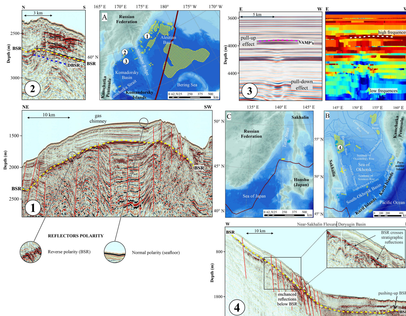
Figure 4. Gas hydrate accumulations of filtration origin in the Far Eastern Seas off Russia; numbers in circles represent positions of hydrate-related anomalies on seismic sections. Symbols are shown in Figure 3.
